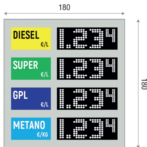
DISPLAY A LED H CIFRA 30 CM
